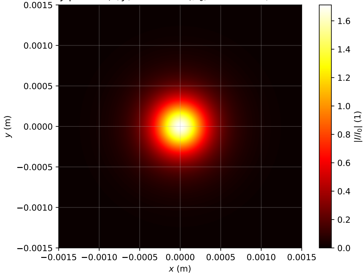
Intensity profile I(x, y, z = 1.274m)/I_0 , Pin=1.0Pcr, artificial time
